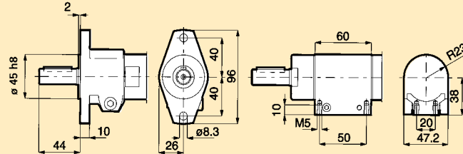
Optional Mountings
